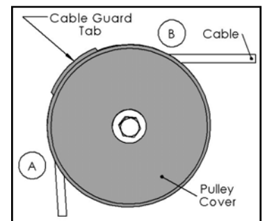
Pulley Cover BFM-50345
