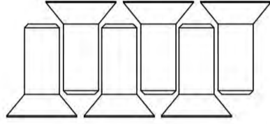
FHSCS 3/8" x 1" (QTY=6)
